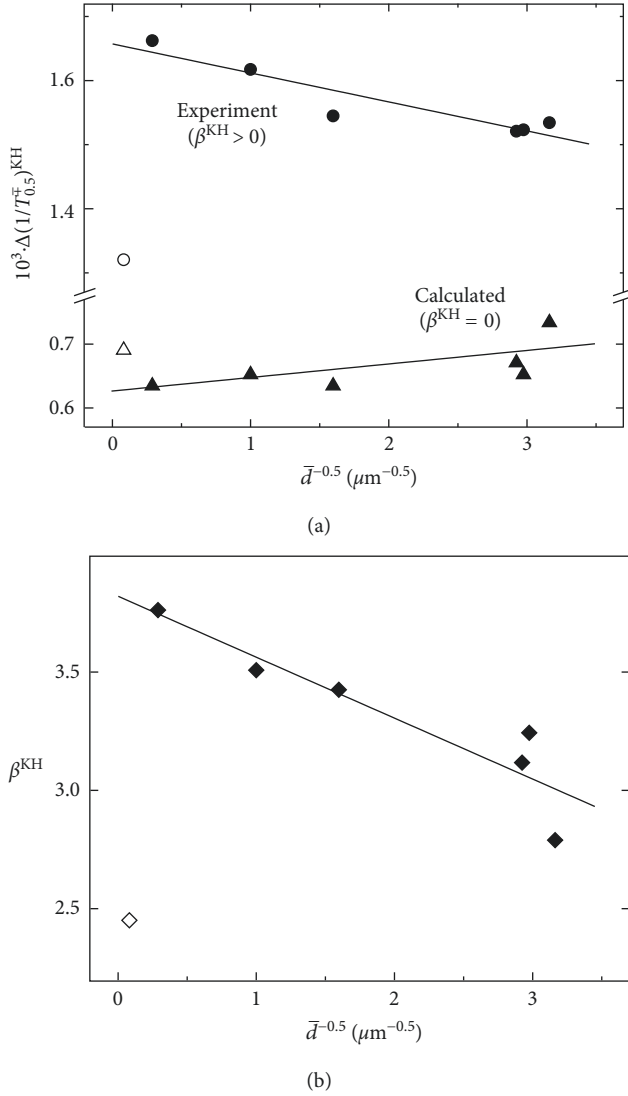
FIGURE 6: Dependences of (a) the experimentally measured width \Delta(1/T_{0.5}^{\tau})^{\text{KH}} of the KH peak and calculated according to (14) for the case \beta^{\text{KH}}=0 and (b) the distribution parameter \beta^{\text{KH}} on the mean grain size \bar{d} . Full symbols are the data of the present work; open symbols are the processed data of the work [7].
