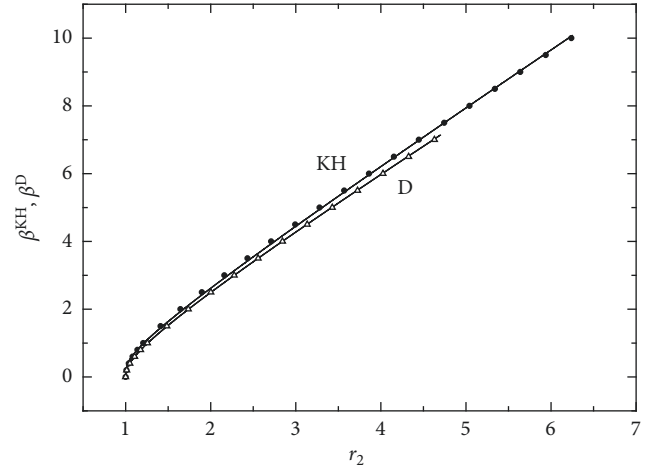
FIGURE 5: The relationship between the value of r_2 and the distribution parameters for the Koiwa–Hasiguti peaks \beta^{\text{KH}} (the present work) and for the Debye peaks \beta^{\text{D}} (the data from [14] were processed). The points correspond to numerical calculations; the solid lines show the approximations \beta^{\text{KH}}(r_2) and \beta^{\text{D}}(r_2) ((25) and (26), resp.).
