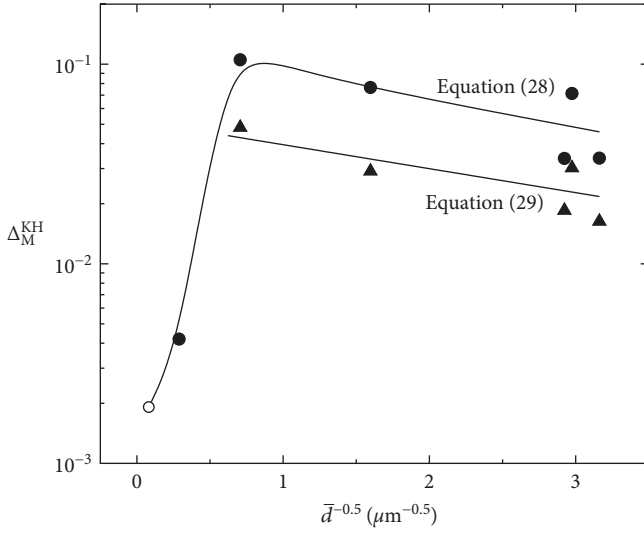
FIGURE 8: Dependences of the relaxation strength \Delta_M^{\text{KH}} on the mean grain size \bar{d} obtained from the KH peak height (Equation 28) and from the measurements of the dynamic Young's modulus (29).
