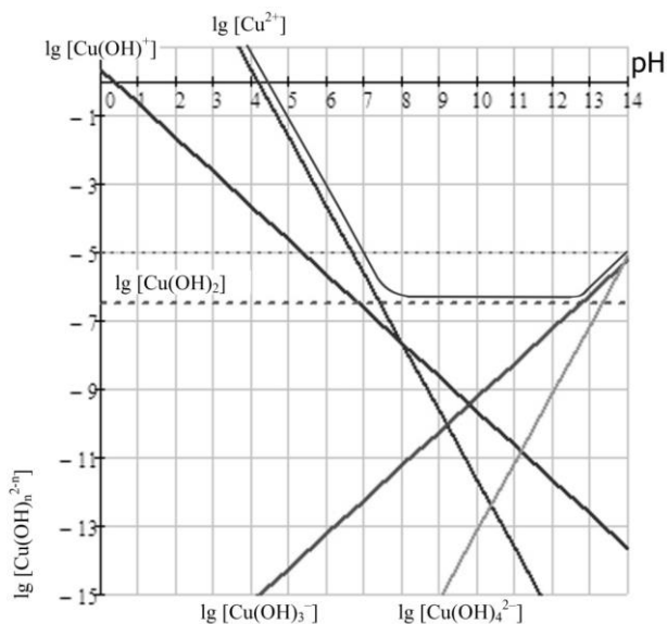
Figure 1 – The concentration-logarithmic diagram (CLD) of forming copper hydroxocomplexes
