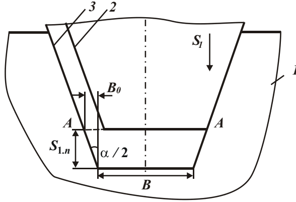
Fig. 1. The calculation scheme of gear grinding parameters by the profile copy method: 1 – gear; 2, 3 – grinding wheel positions at (n-1) and n passes.
